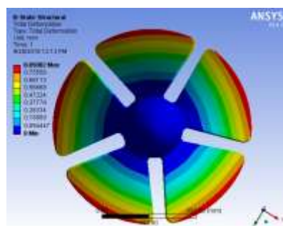
Fig.4.12: Deformation
