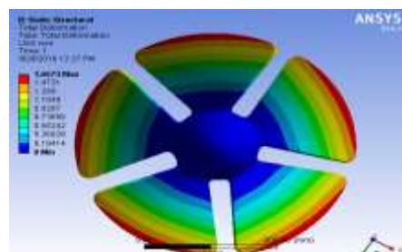
Fig.4.9: Deformation
