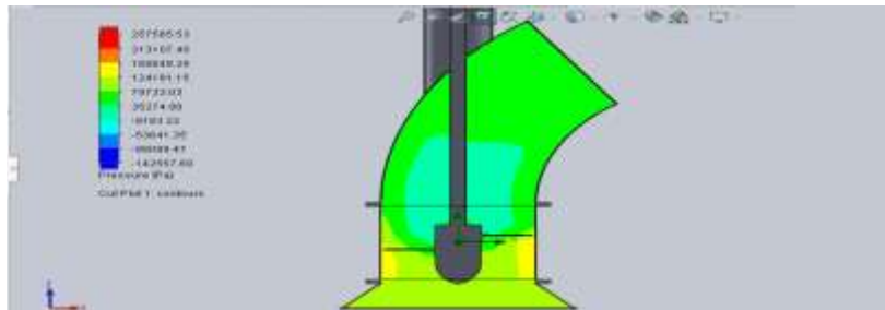
Fig.4.16: Pressure variation
