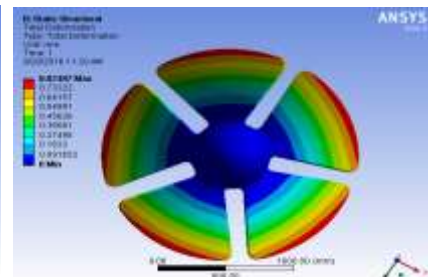
Fig.4.4: Deformation
