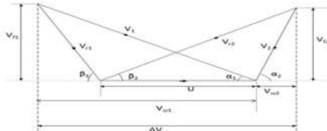
Fig.2.1: Velocity triangle
