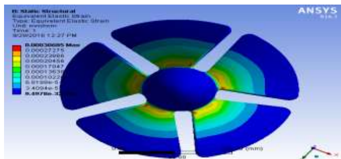
Fig.4.10: Elastic strain
