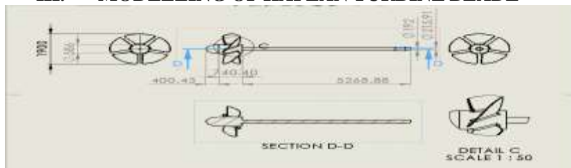
Fig.3.1: Drawing of a turbine blades along with shaft
