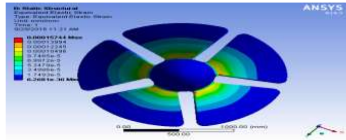
Fig. 4.5: Elastic strain
