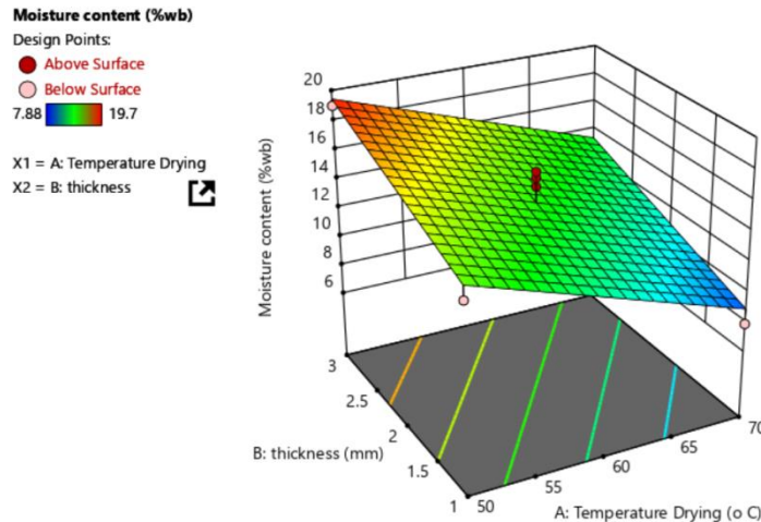
Figure 4. Three-dimensional surface graph of moisture content response
