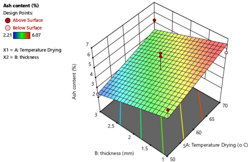
Figure 8. Three-dimensional surface graph of ash content response
